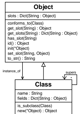
Figure 1: Core Converge data model.
