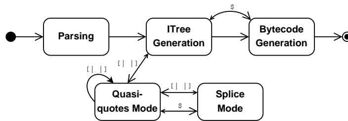
Figure 2: Convergence compiler states.
