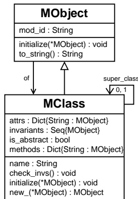
Figure 4: TM data model.
