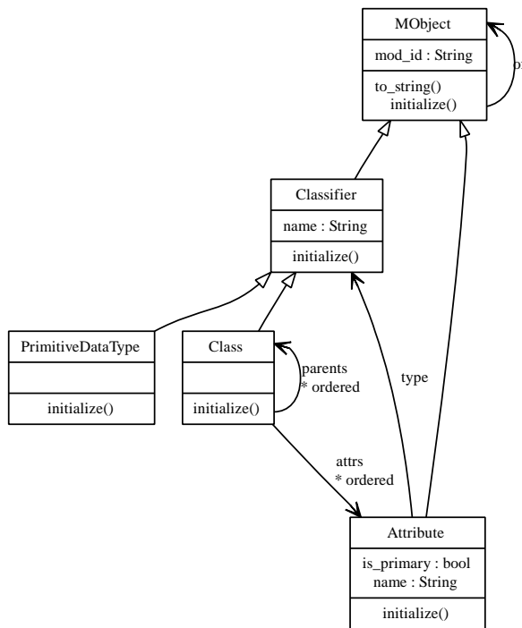
Figure 5: ‘Simple UML’ modelling language visualized.
