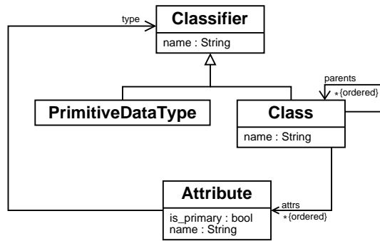
Figure 3: ‘Simple UML’ model.
