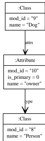
Figure 6: A ‘Simple UML’ model language visualized.
